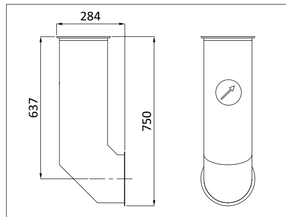
PIPE WITH FLOW INDICATOR FOR AFU 1200
