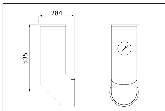
PIPE WITH FLOW INDICATOR FOR AFU 900
