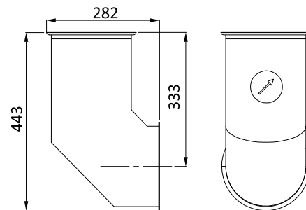
PIPE WITH FLOW INDICATOR FOR AFU 300
