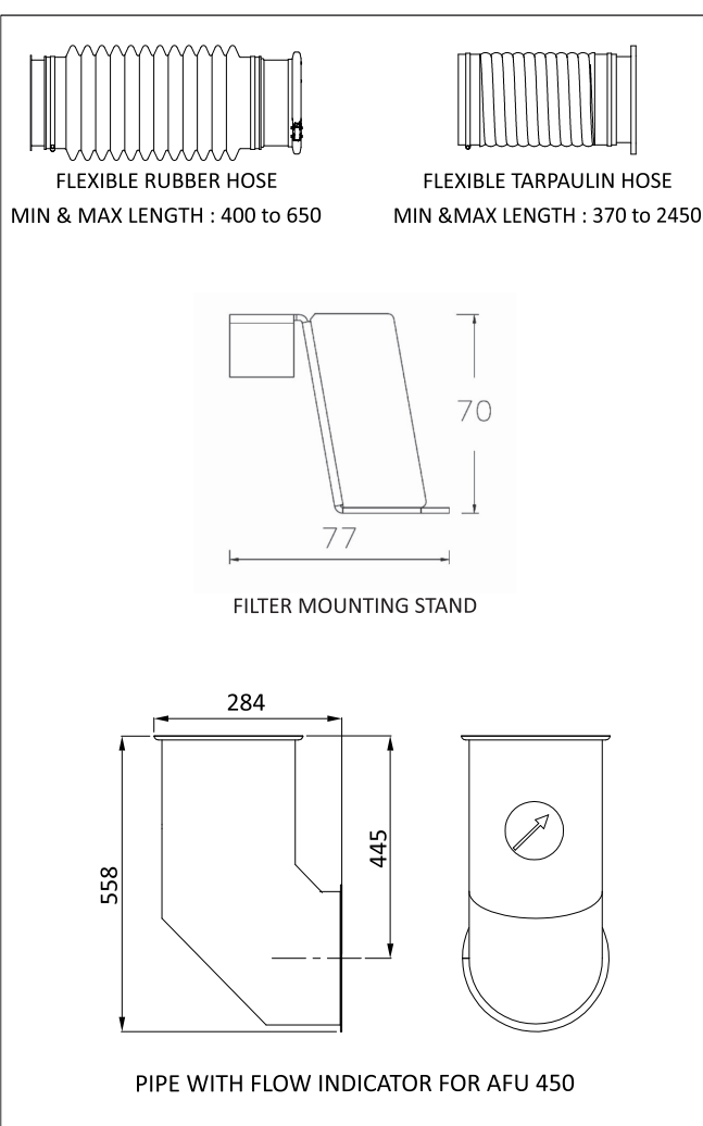
OPTIONAL KIT FOR FLOOR MOUNTING
