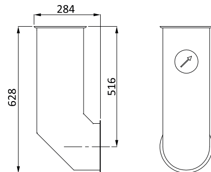
PIPE WITH FLOW INDICATOR FOR AFU 600
