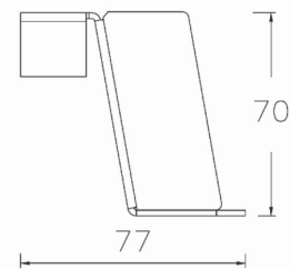
FILTER MOUNTING STAND
